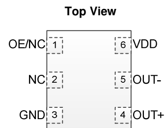
Figure 1. Pin Assignments
