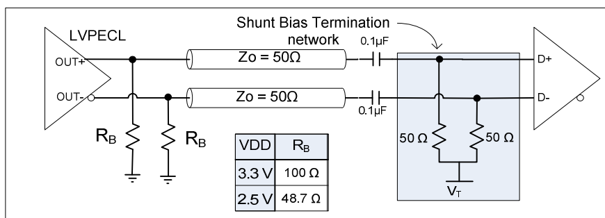
Figure 5: LVPECL with AC-coupled termination
