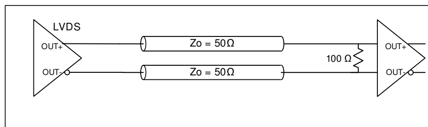
Figure 9: LVDS single DC termination at the load
