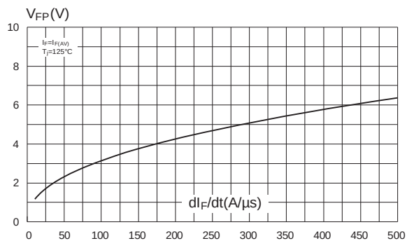
Figure 9: Transient peak forward voltage versus dI_F/dt (typical values, per diode) (TO-220AB)
