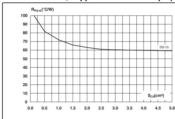
Figure 15. Thermal resistance, junction to ambient, versus copper surface under each lead - DO 15 (Epoxy FR4, copper thickness = 35 μm)
