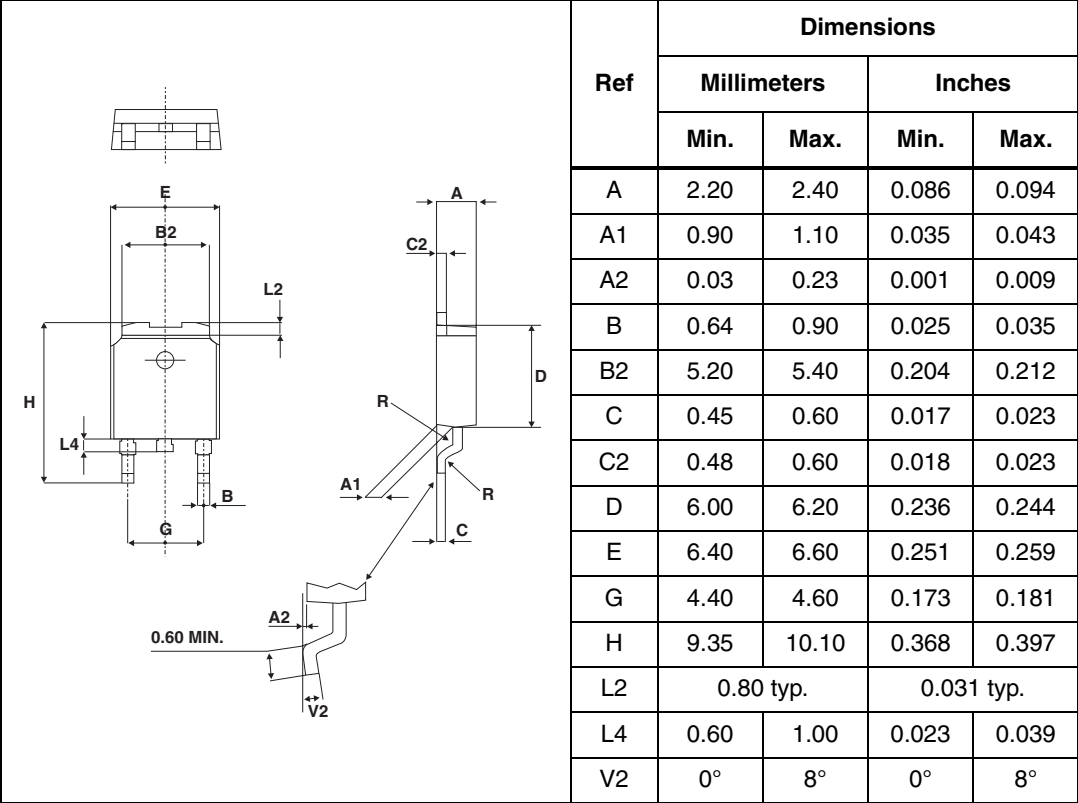
Figure 11. DPAK dimensions
