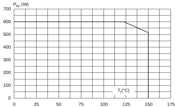
Figure 3: Peak pulse power dissipation versus initial junction temperature
