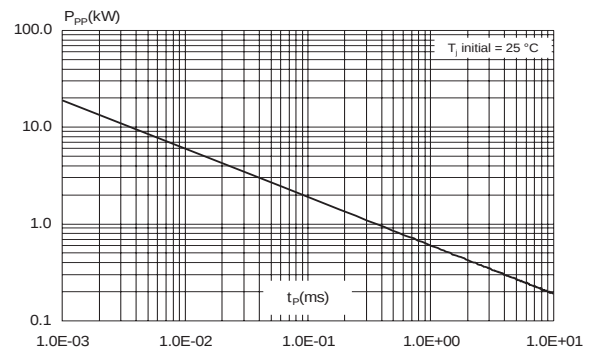
Figure 4: Peak pulse power versus exponential pulse duration ( T_{amb} = 25^\circ\text{C} )
