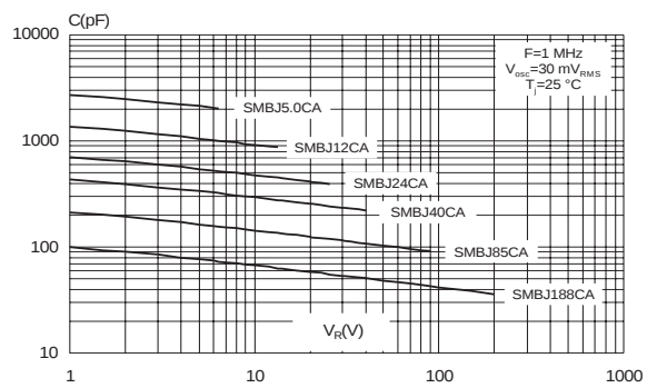
Figure 7: Junction capacitance versus reverse applied voltage (typical values) (SMBJxxCA)
