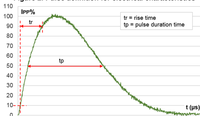
Figure 2: Pulse definition for electrical characteristics
