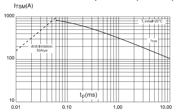
Figure 6: Non repetitive surge peak on-state current versus sinusoidal pulse width ( t_p < 10 ms)
