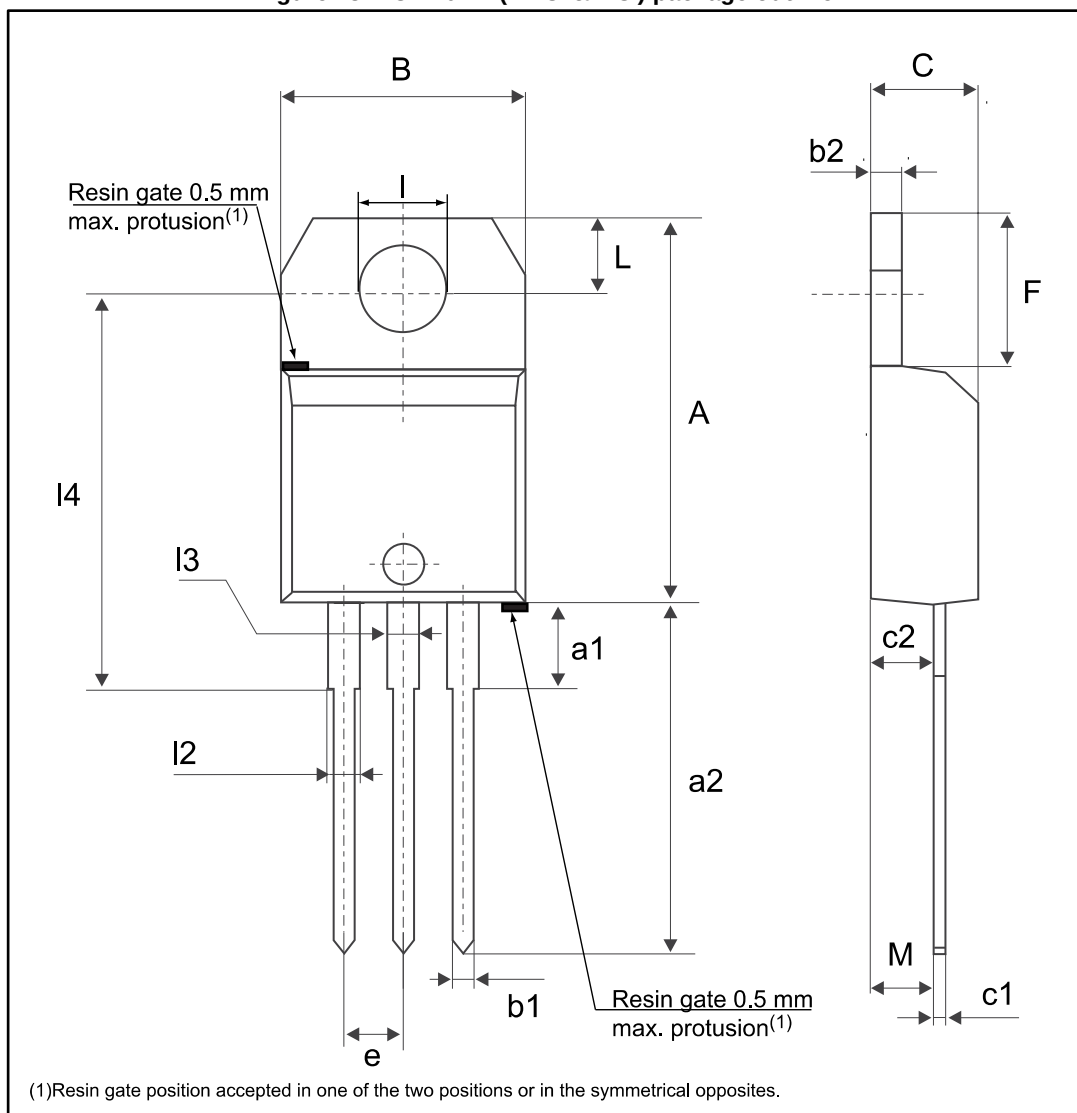
Figure 13: TO-220AB (NIns. &amp; Ins.) package outline
