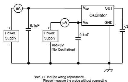
Current consumption measurement
