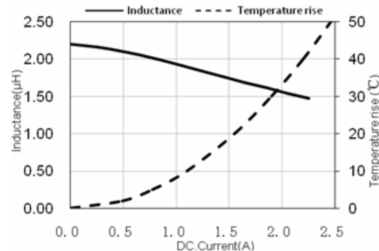
ASPI-U201610-2R2
