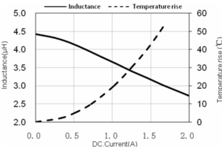
ASPI-U201610-4R7
