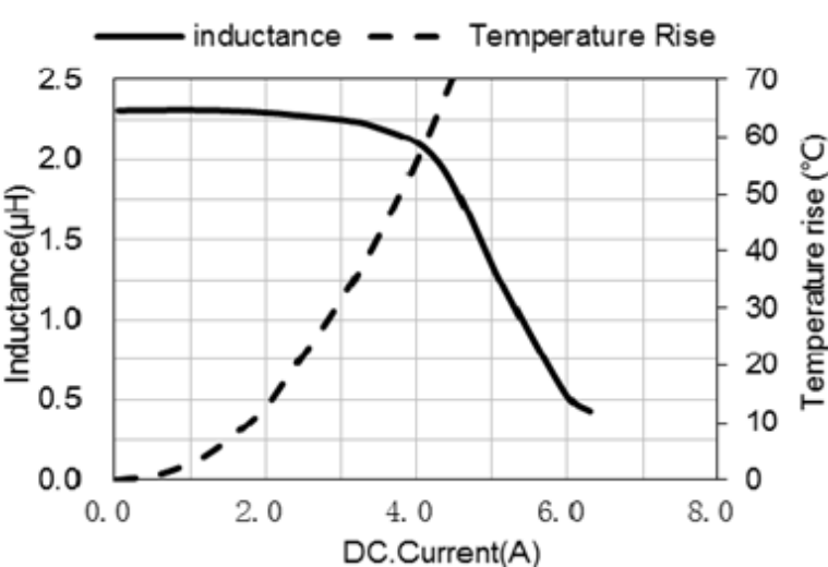
ASPIAIG-S4035-2R2
