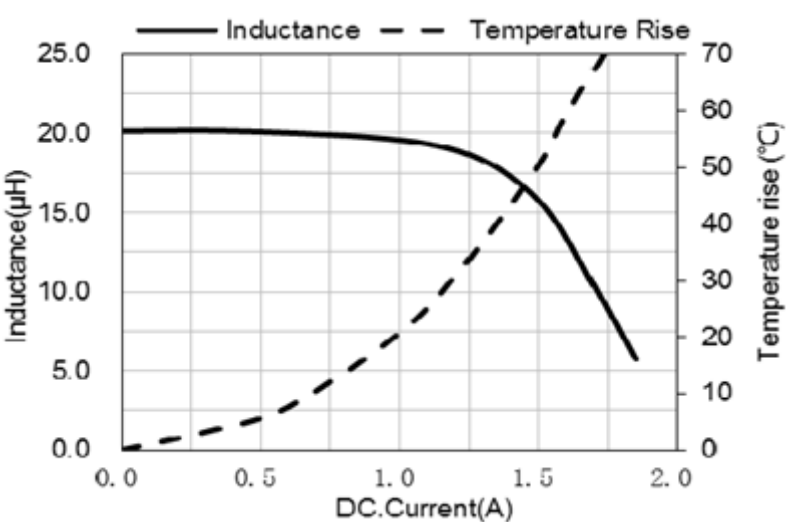
ASPIAIG-S4035-220
