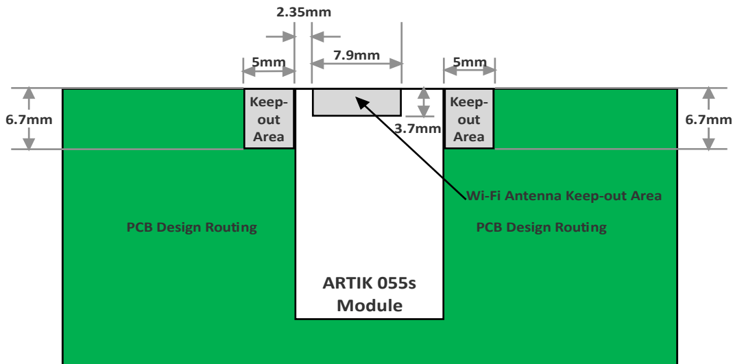
Figure 6. Module Placement Restrictions
