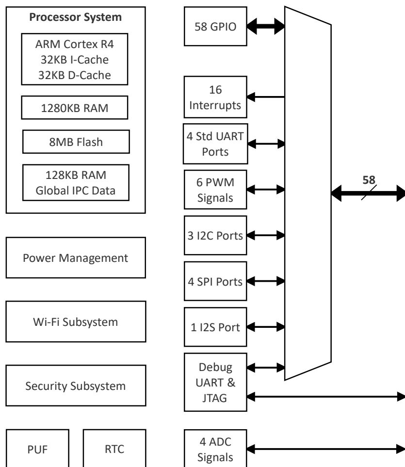
Figure 2. ARTIK 055s Module Block Diagram
