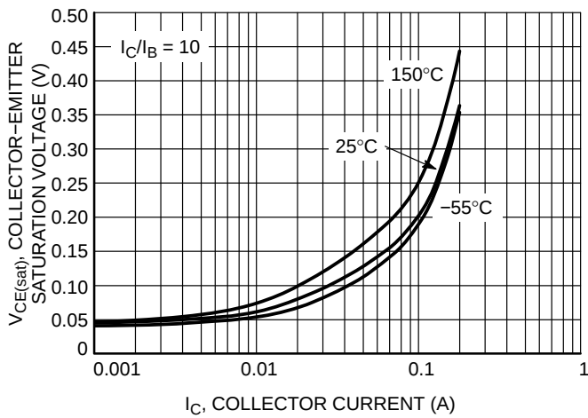
Figure 34. Collector Emitter Saturation Voltage vs. Collector Current
