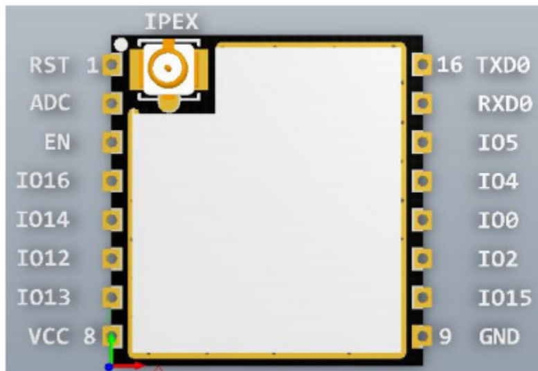
Figure 2 ESP-07S pinout
