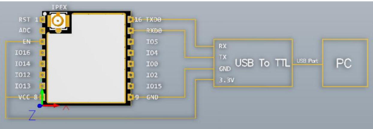
Figure 7 ESP-07S connect with computer
