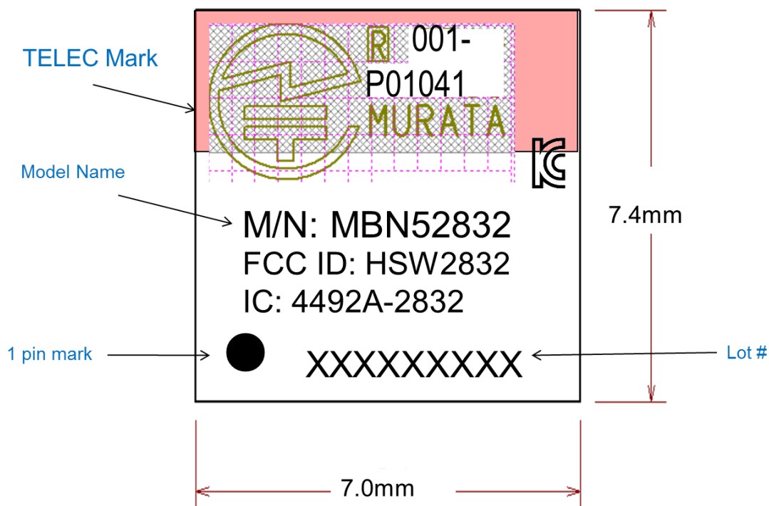
Figure 10.7 Module Marking Diagram
