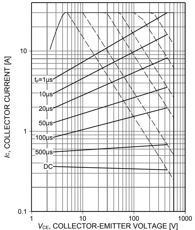
Figure 2. Forward bias safe operating area ( D = 0 , T_C = 25^\circ C , T_{vj} \leq 175^\circ C ; V_{GE} = 15V )
