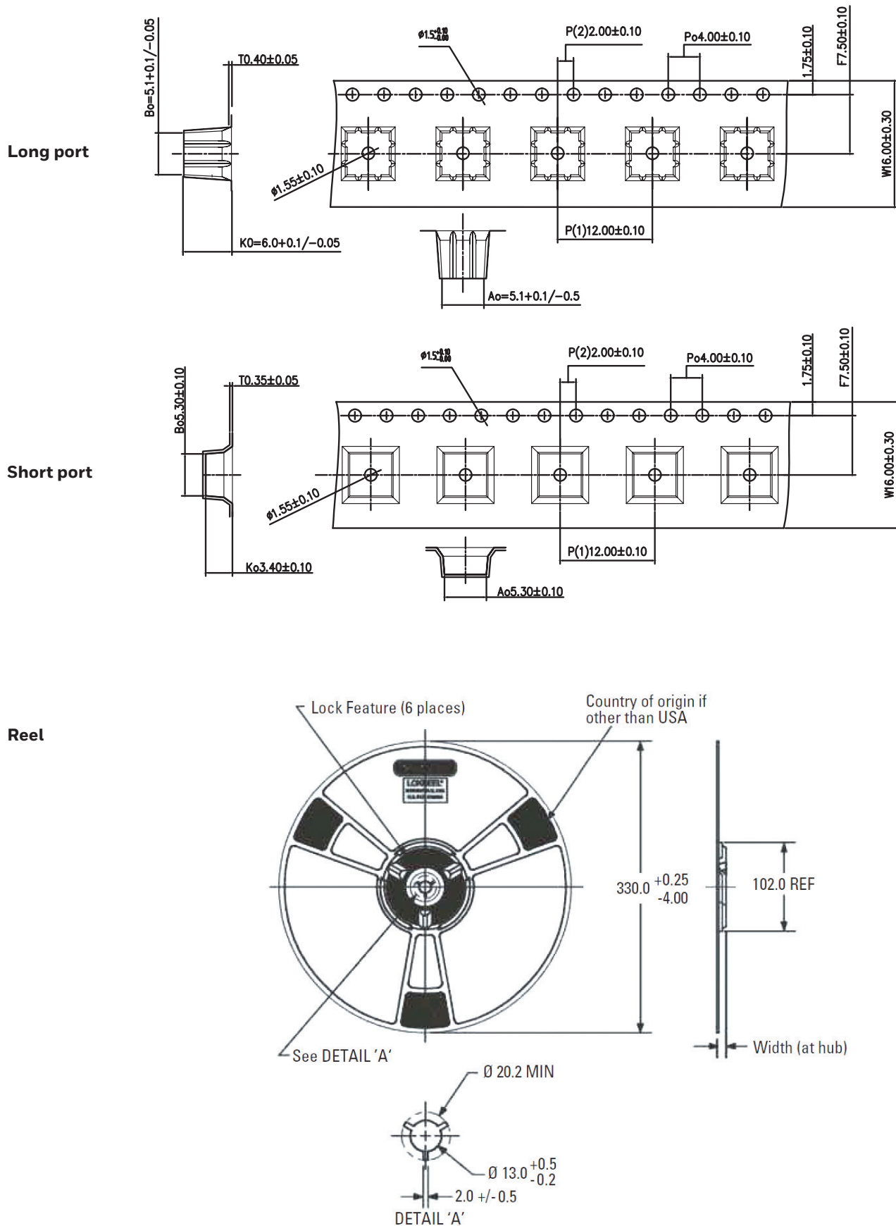
Figure 11. Product Tape and Reel Dimensions (For reference only: mm.)
