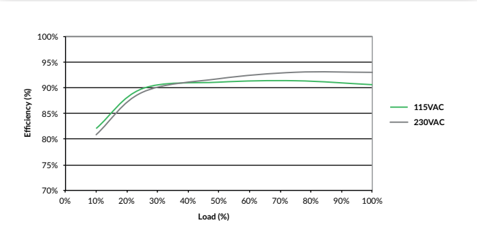
Figure 4 GCU500PS48
