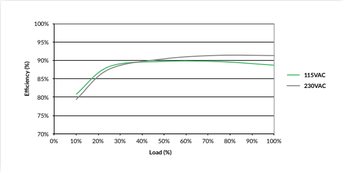
Figure 3 GCU500PS24
