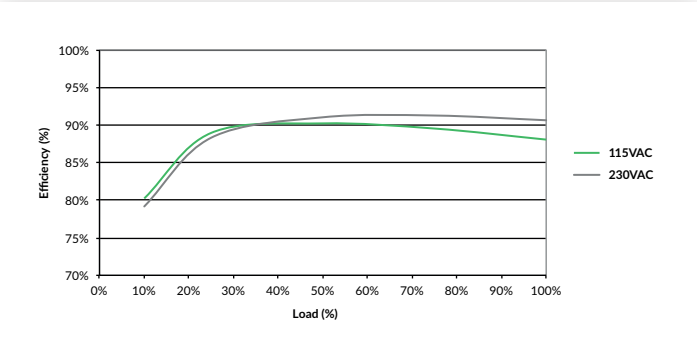
Figure 2 GCU500PS12
