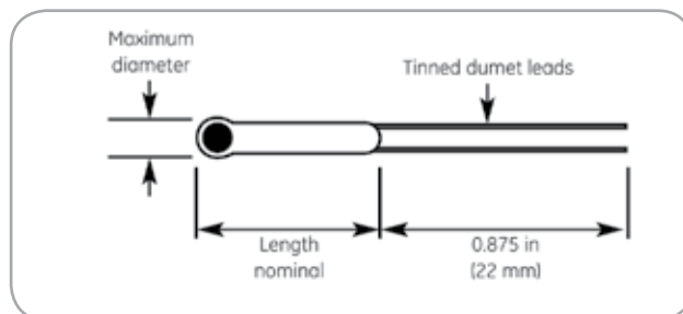
NTC Types 60/65/85/100 dimensions
