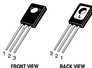
TO-225 CASE 077 STYLE 1
