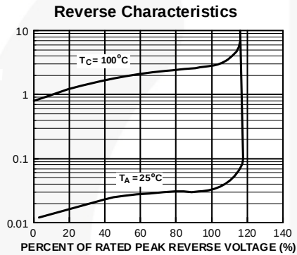
Figure 3. Reverse Characteristics
