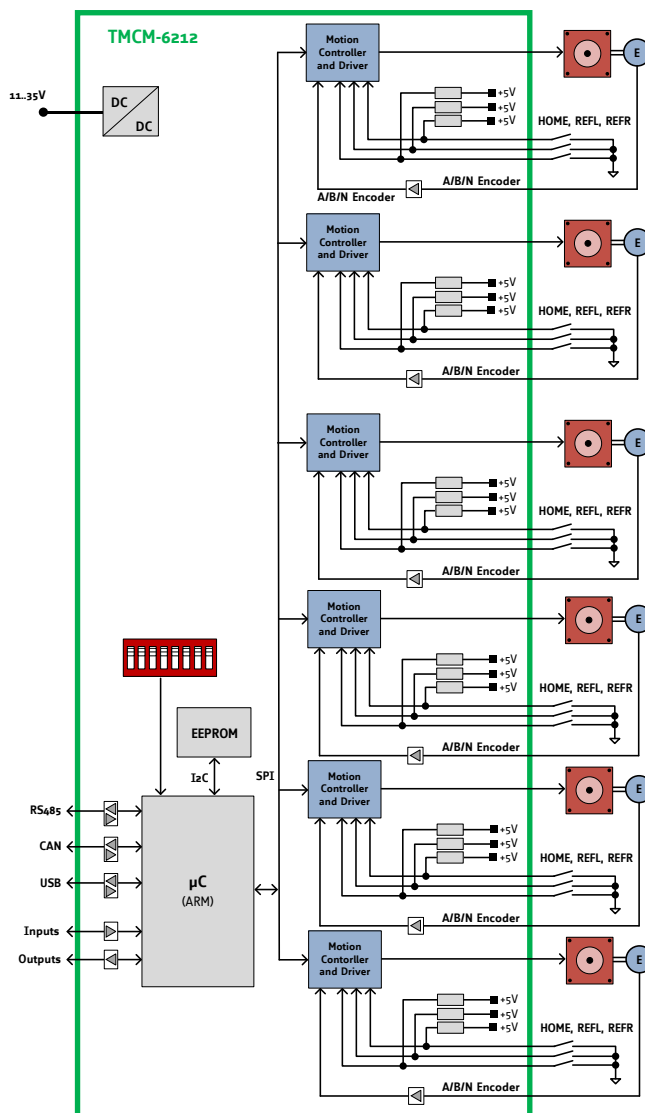
Figure 10.1 Main parts of the TMC6212
