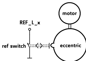
Figure 3.6 One reference switch
