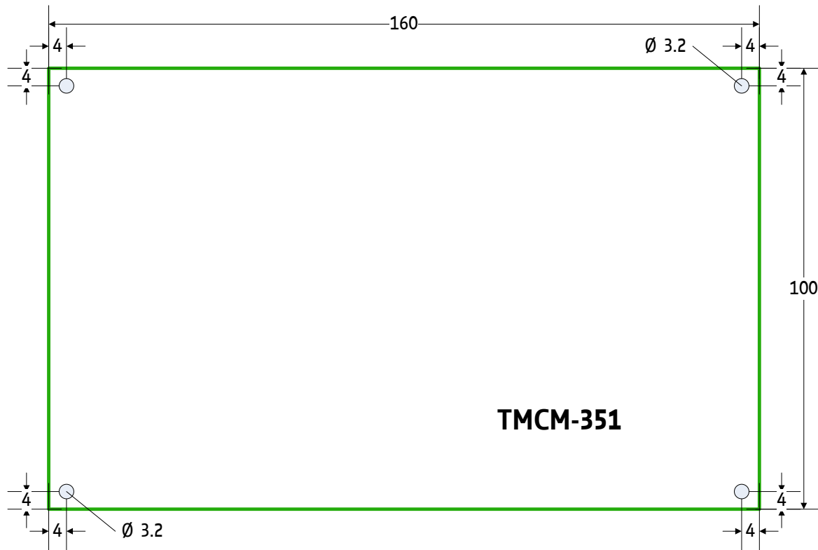
Figure 3.1 Dimensions of TMC351
