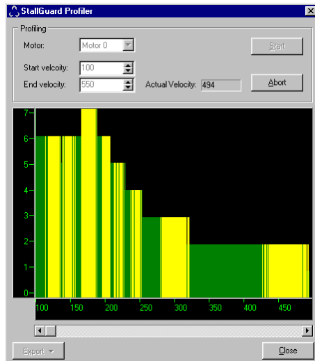
Figure 7.7: The stallGuard™ profiler
