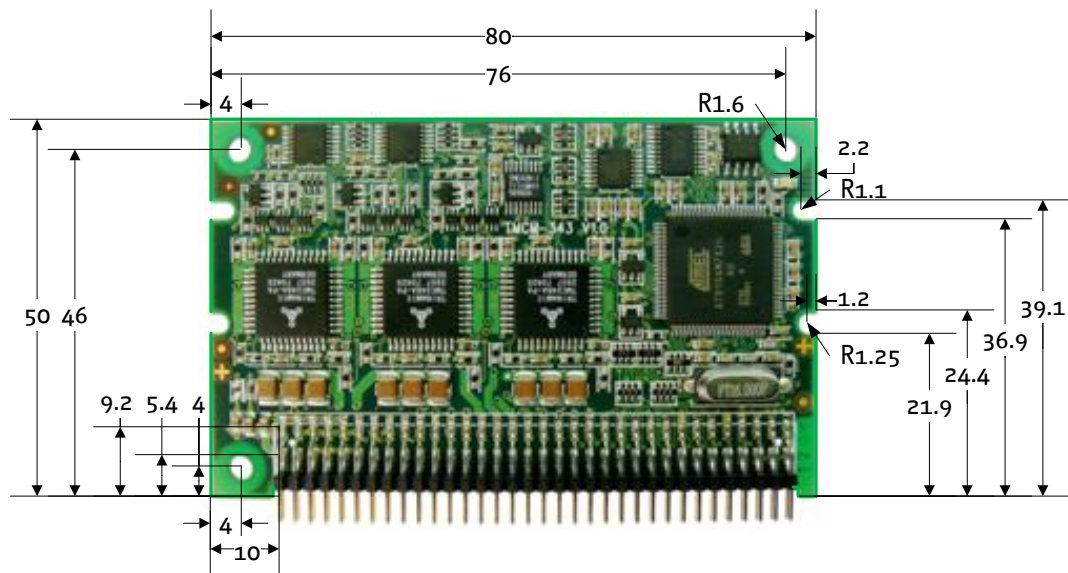
Figure 5.1: Front view of TCMC-343 (all values in mm)
