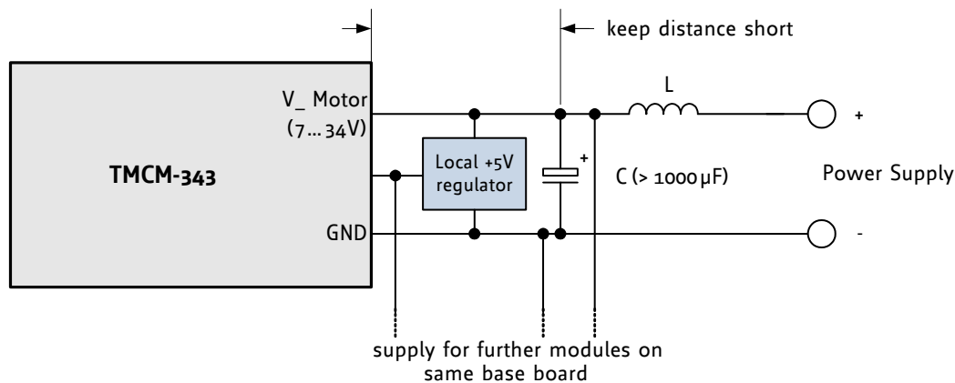
Figure 5.4: Power supply requirements for TMCM-343
