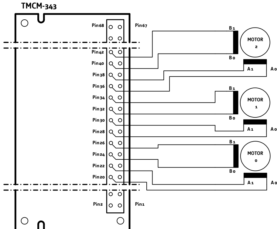
Figure 7.2: Connecting the motors
