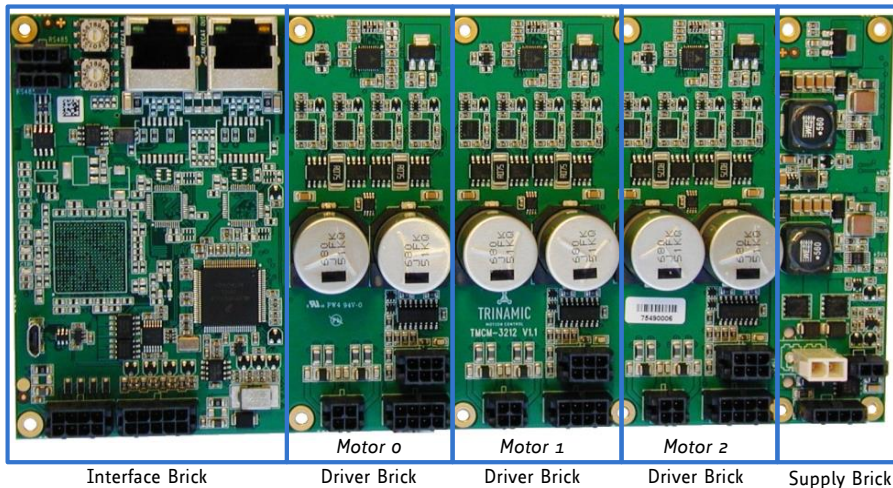
Figure 5.1 different bricks used for the TMC3212 / TMC3213
