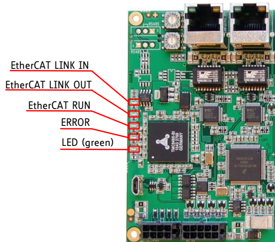
Figure 7.3: LEDs on TMC3213 interface brick
