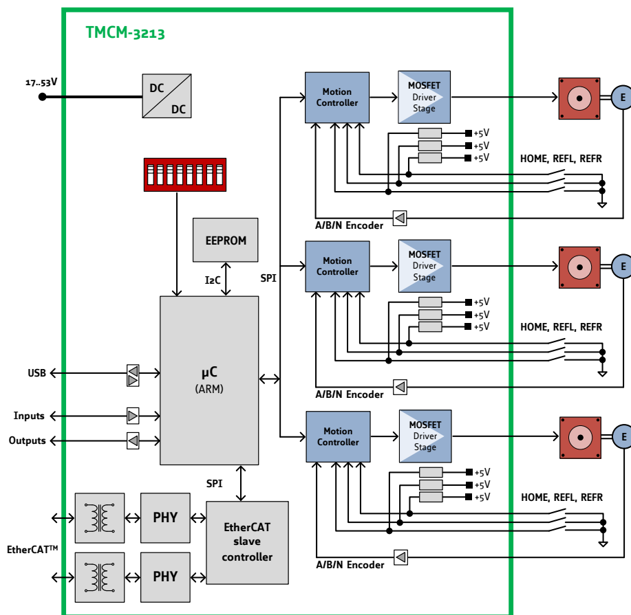
Figure 11.1 Main parts of the TMC3213
