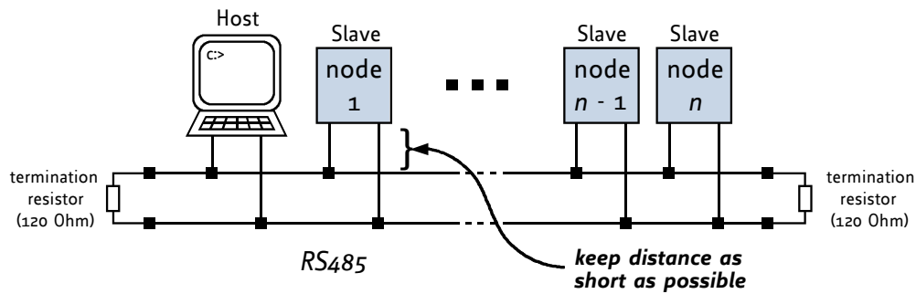
Figure 5.3: Bus structure
