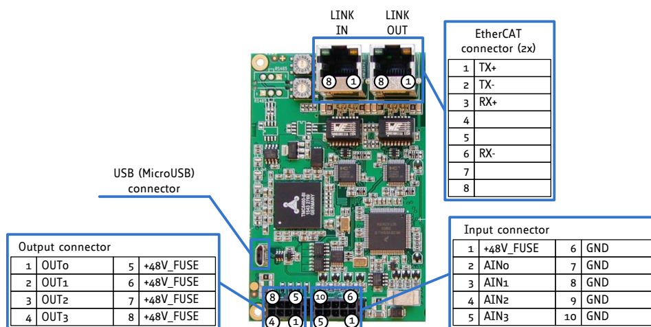
Figure 5.3 TMC-3213 interface brick
