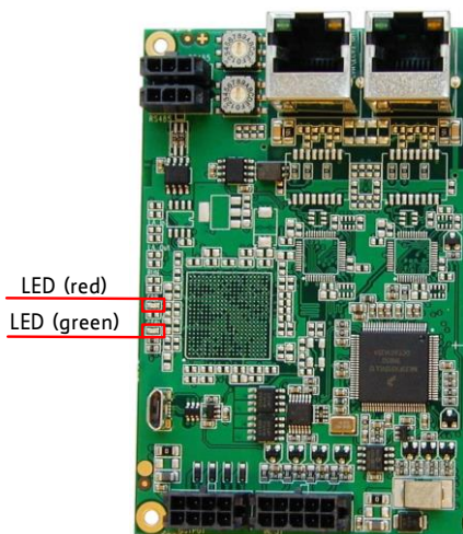
Figure 7.2: LEDs on TMC3212 interface brick
