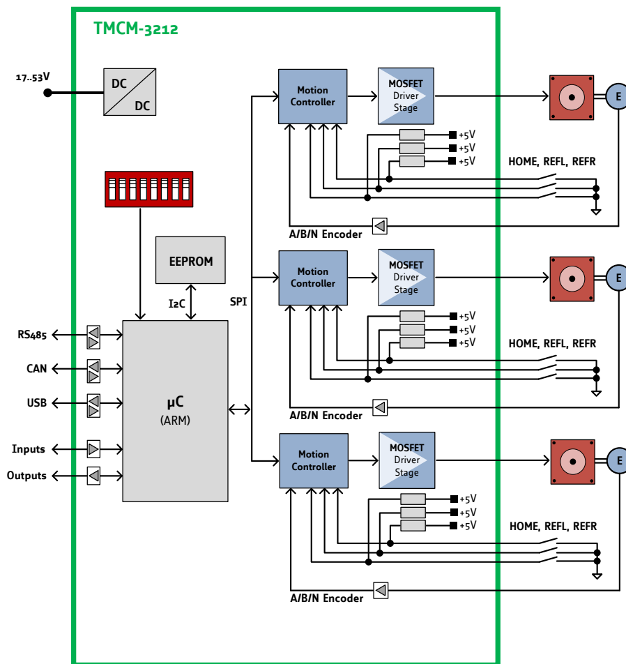
Figure 10.1 Main parts of the TMC3212
