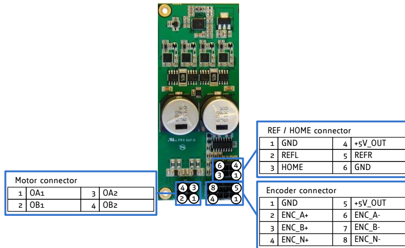
Figure 5.4 TMC3212 + TMC3213 Driver Brick
