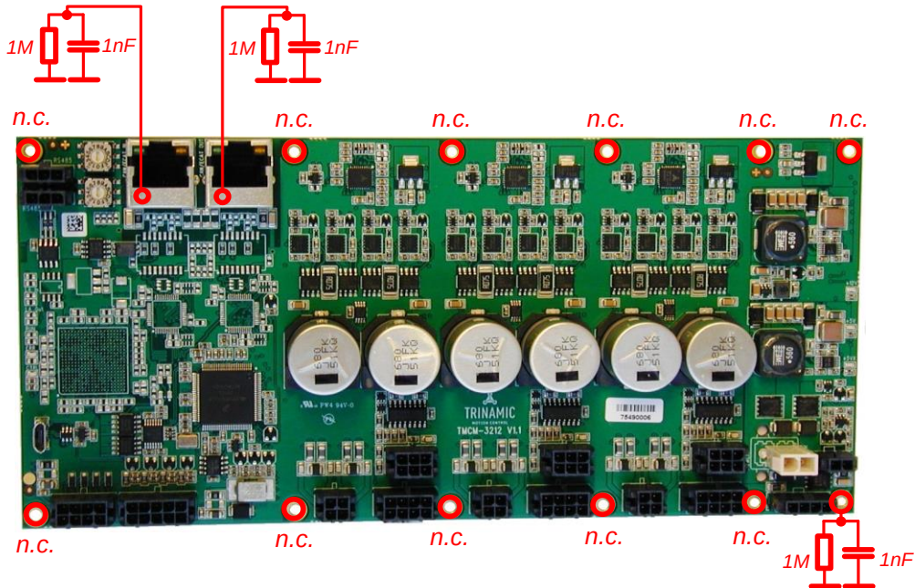
Figure 4.2 TMC3212 / TMC3213 mounting hole connections
