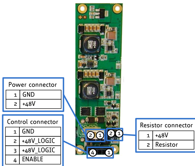
Figure 5.5: TMC3212 + TMC3213 Power supply Brick
