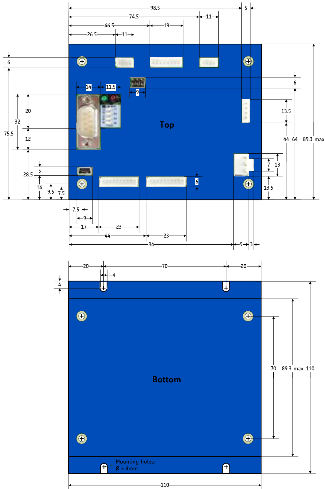
Figure 3.1 Dimensions of TMC-1311 (all values in mm).
