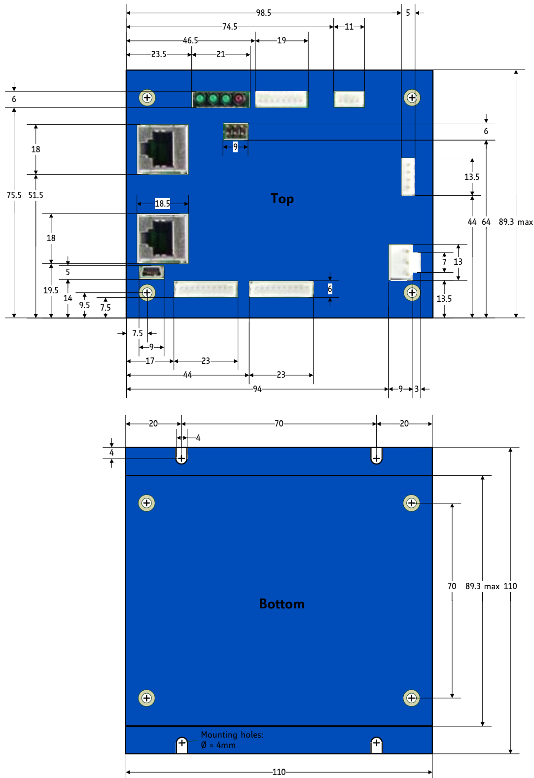
Figure 3.1 Dimensions of TMC-1310 (all values in mm)
