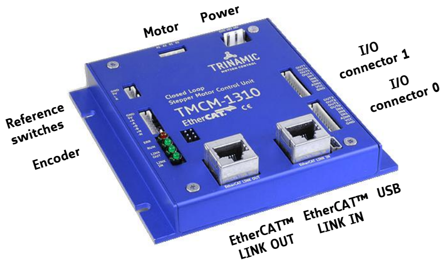
Figure 3.2 TMC-1310 connectors
