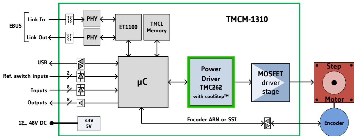
Figure 6.1 Main parts of TMC-1310
