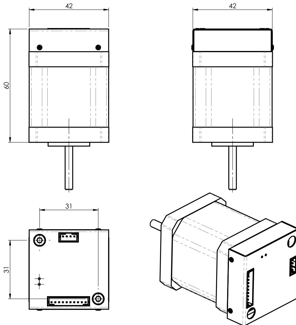
Figure 7: TCM-1270 mechanical dimensions with a NEMA17 stepper motor
