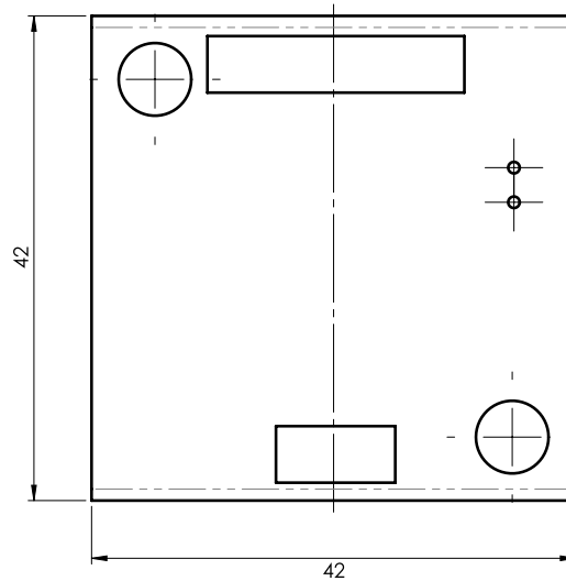
Figure 6: TCM-1270 top view mechanical dimensions
