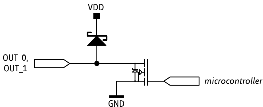
Figure 3.7 General purpose outputs
