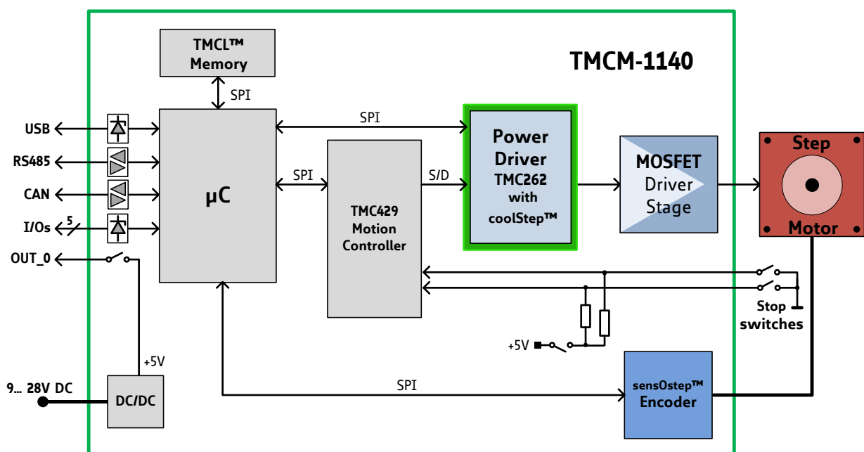
Figure 8.1 Main parts of the TMC1140
