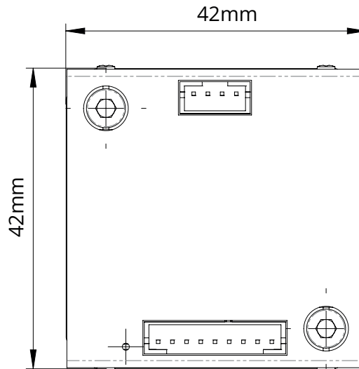
Figure 5: TCM-1070 top view mechanical dimensions
