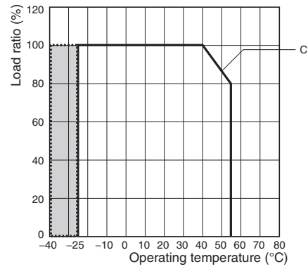
(C) Front, Side-by-side mounting
