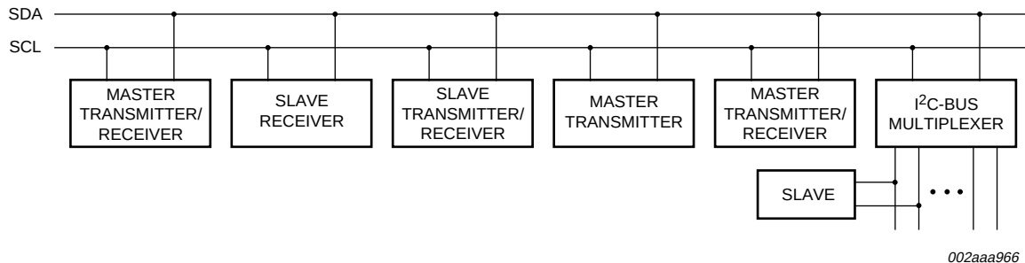
Fig 16. System configuration
