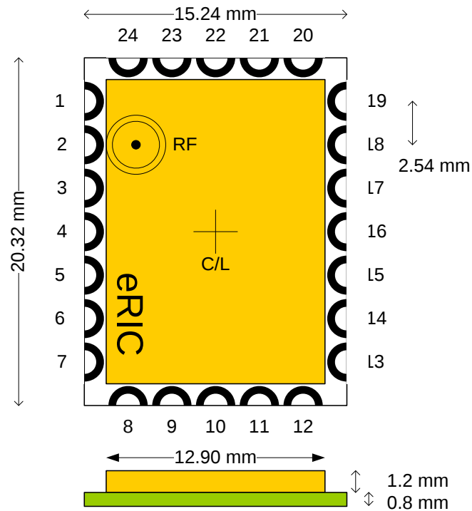
Figure 1 Mechanical Drawing
