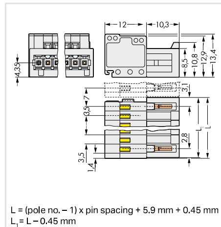
1-conductor male connector, light gray, 3.5 mm (0.138 inch) pin spacing
