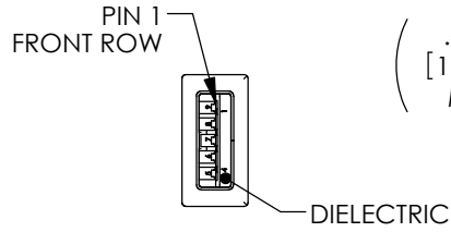
"P1" USB 3.0 SERIES "A" PLUG CONTACTS 30μ GOLD
