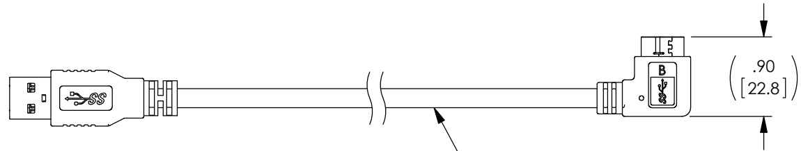
"P2" USB 3.0 SERIES "MICRO B" RIGHT ANGLE PLUG CONTACTS 30μ GOLD
