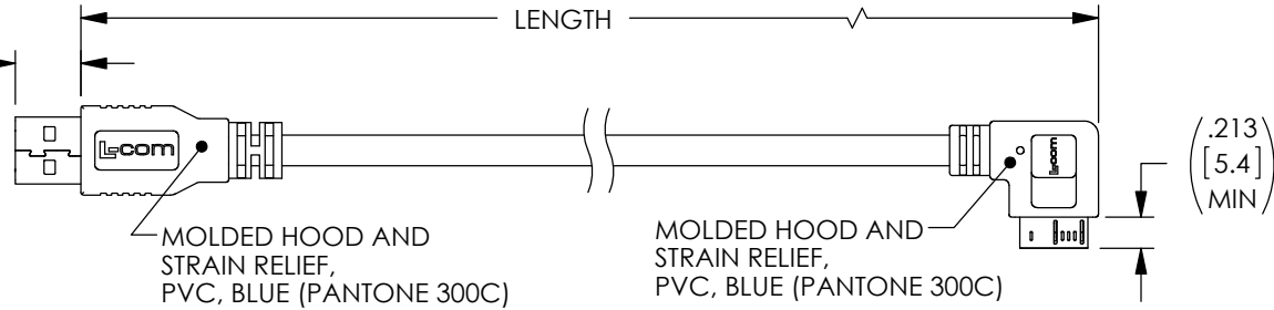
"P2" USB 3.0 SERIES "MICRO B" RIGHT ANGLE PLUG CONTACTS 30μ GOLD
