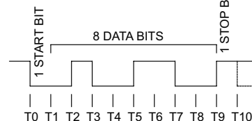
Figure 13, Data Format - 8 Data Bits
