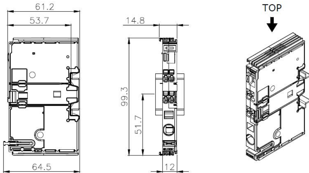
Figure 4-4: EasyB dimensions
