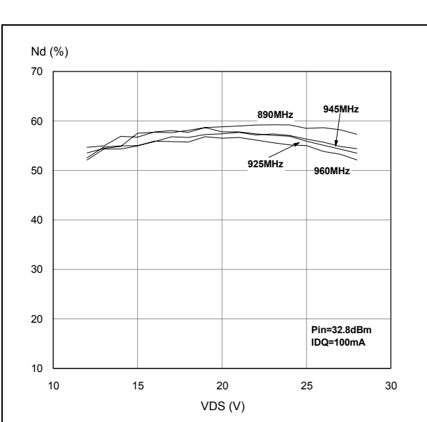
Figure 13. Drain efficiency vs supply voltage
