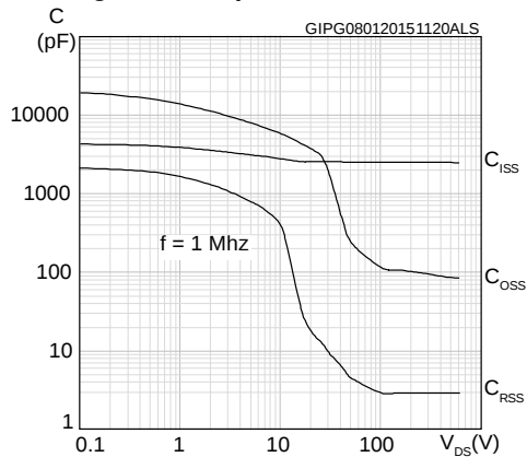
Figure 10: Capacitance variations
