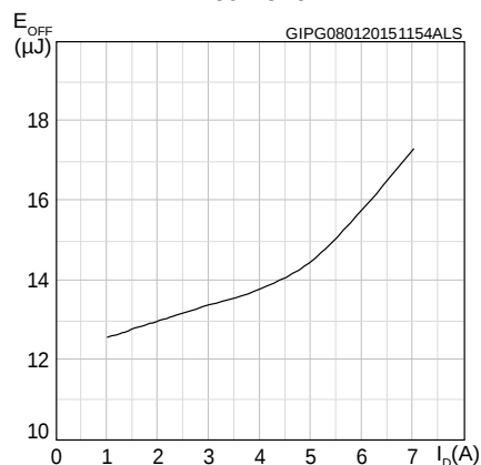
Figure 12: Turn-off switching loss vs drain current
