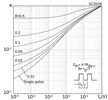
Figure 3: Thermal impedance for D 2 PAK and TO-220
