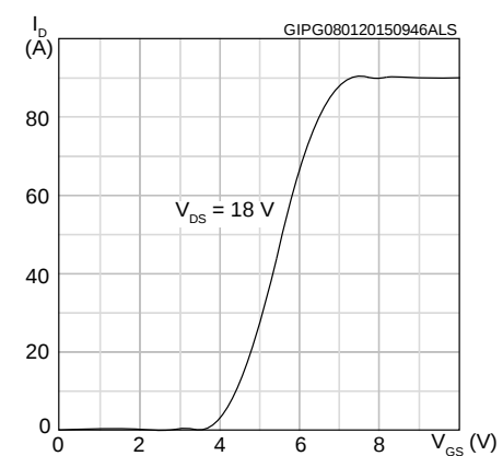
Figure 7: Transfer characteristics
