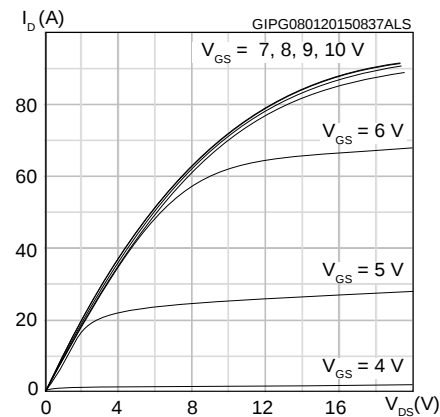
Figure 6: Output characteristics
