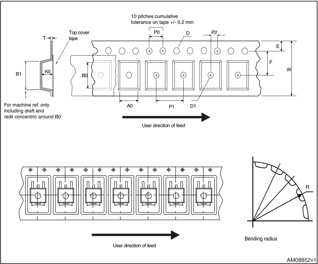
Figure 30. Tape
