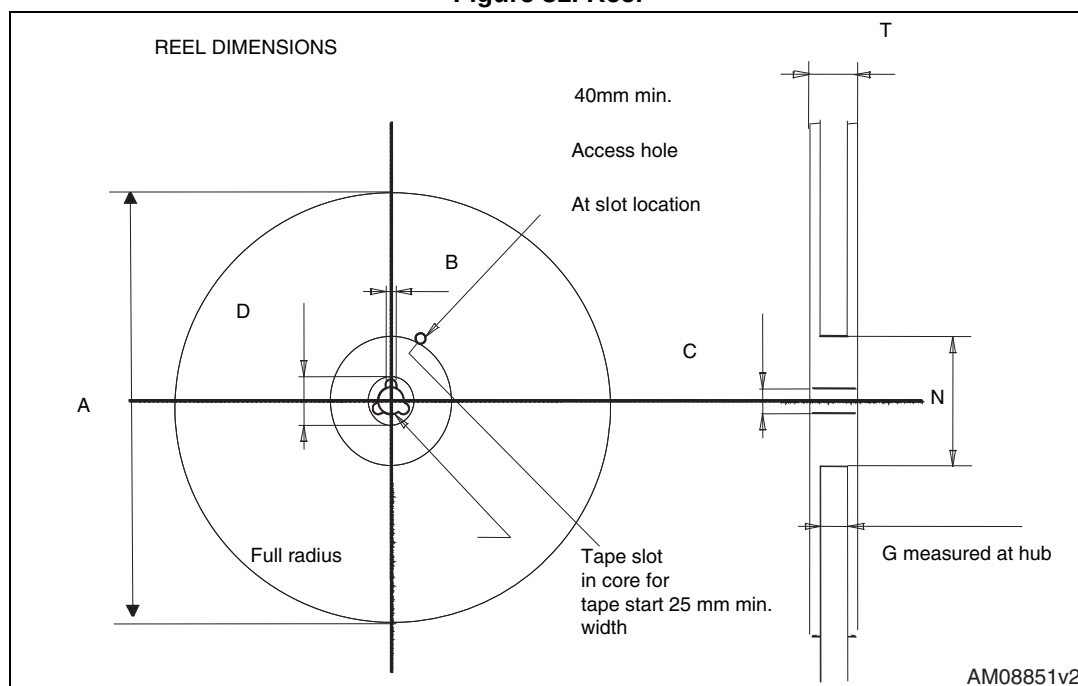
Figure 31. Reel
