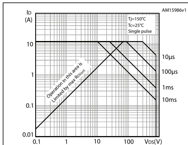
Figure 2. Safe operating area for DPAK and IPAQ
