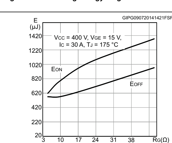
Figure 17. Switching energy vs gate resistance
