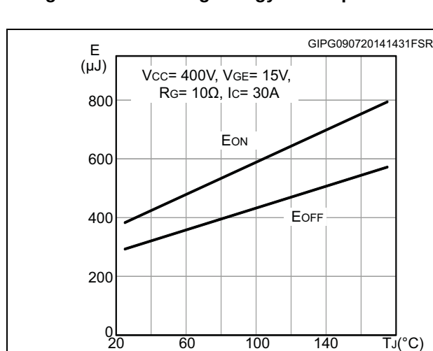
Figure 18. Switching energy vs temperature
