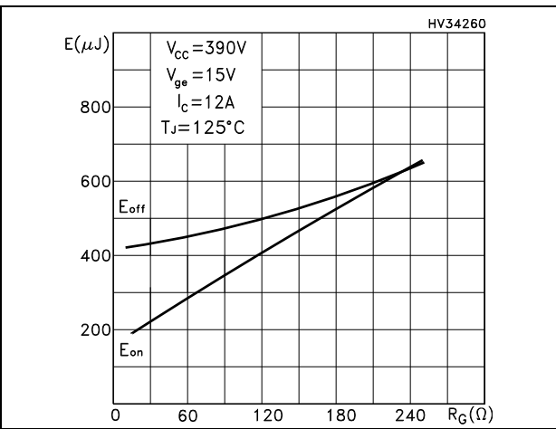
Figure 12. Switching energy vs. gate resistance
