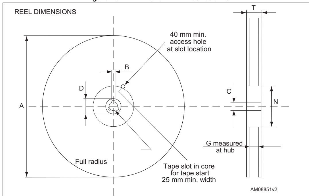
Figure 46. D 2 PAK and DPAK reel outline
