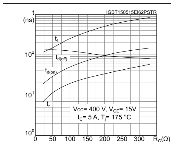
Figure 28. Switching times vs. gate resistance
