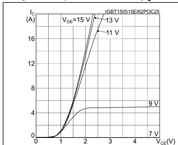
Figure 8. Output characteristics ( T_J = 25^{\circ}\text{C} )
