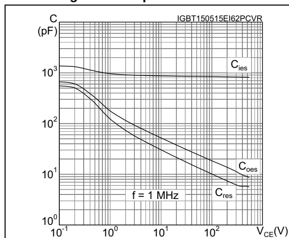
Figure 20. Capacitance variation
