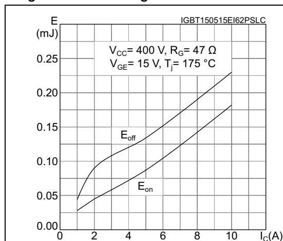
Figure 22. Switching loss vs collector current
