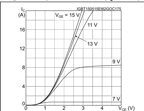
Figure 9. Output characteristics ( T_J = 175^{\circ}\text{C} )
