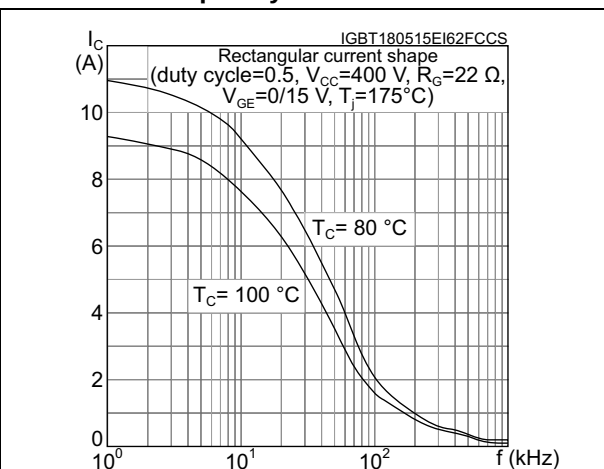
Figure 13. Collector current vs. switching frequency for TO-220FP
