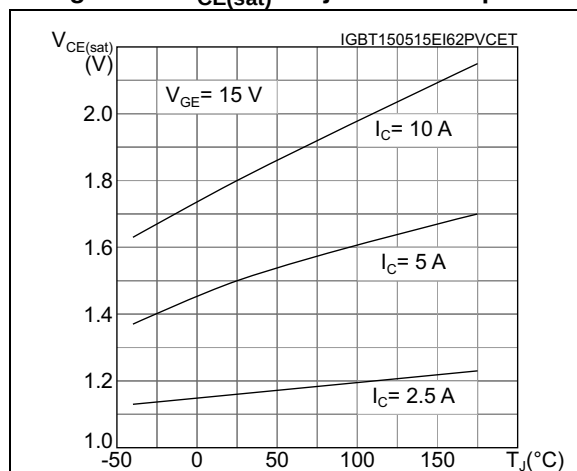
Figure 10. V_{CE(sat)} vs. junction temperature
