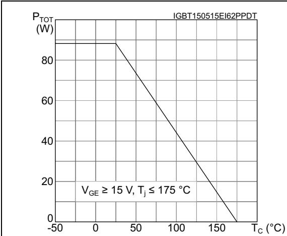
Figure 4. Power dissipation vs. case temperature for DPAK
