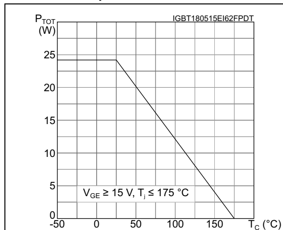
Figure 6. Power dissipation vs. case temperature for TO-220FP
