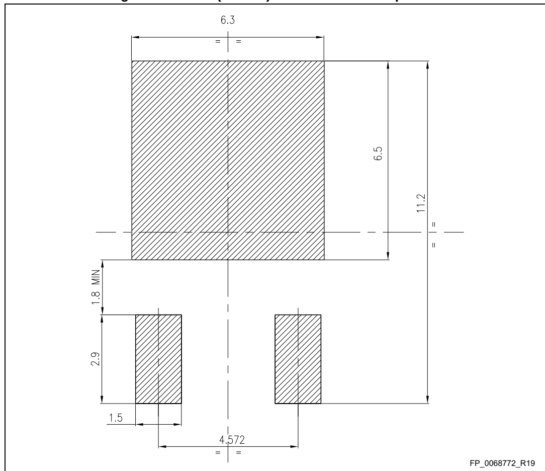
Figure 44. DPAK (TO-252) recommended footprint (b)
