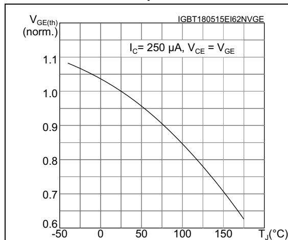
Figure 18. Normalized V_{GE(th)} vs junction temperature
