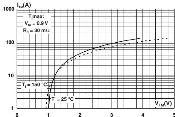
Figure 6. On-state characteristics (maximum values)
