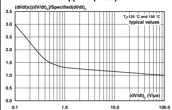
Figure 11. Relative variation of critical rate of decrease of main current (dl/dt)_c versus reapplied (dV/dt)_c
