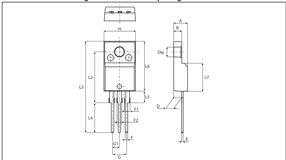
Figure 21. TO-220FPAB package outline
