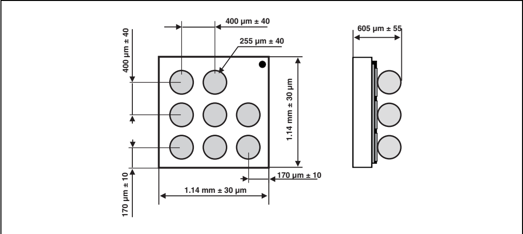
Figure 15. Package dimensions
