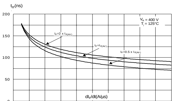
Figure 5: Reverse recovery time versus di_F/dt (typical values)
