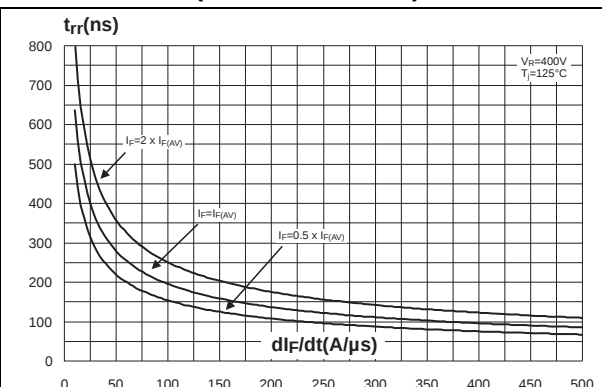
Figure 6. Reverse recovery time versus dl_F/dt (90 % confidence)
