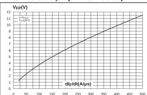
Figure 10. Transient peak forward voltage versus dl_F/dt (90 % confidence)
