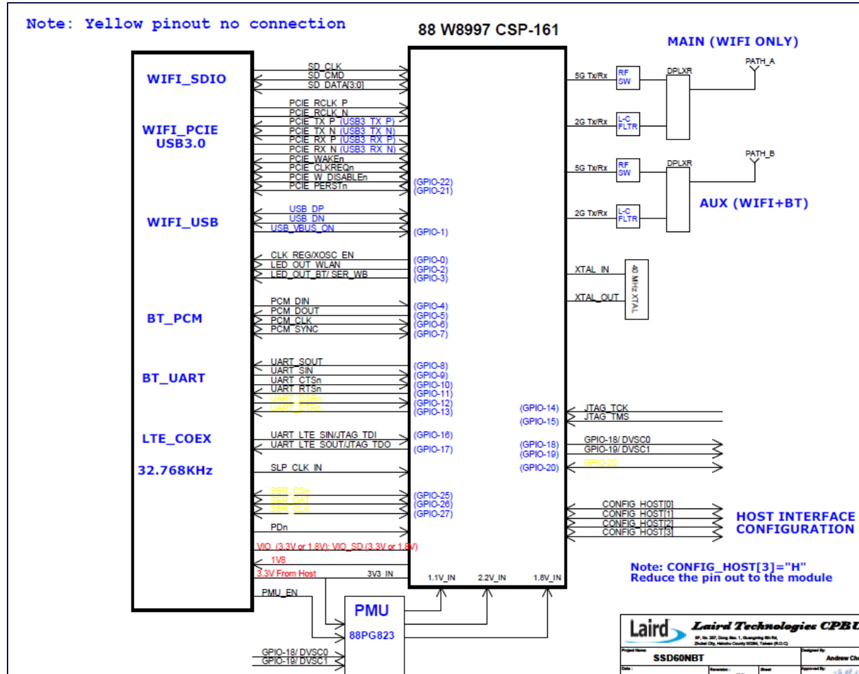
Figure 1: Block diagram
