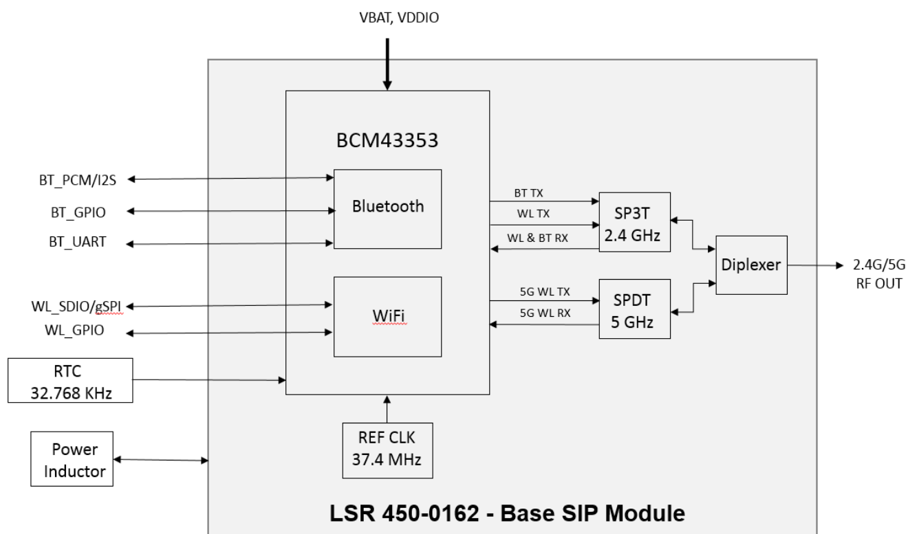
Figure 4 Sterling-LWB5 Base SIP Module Block Diagram
