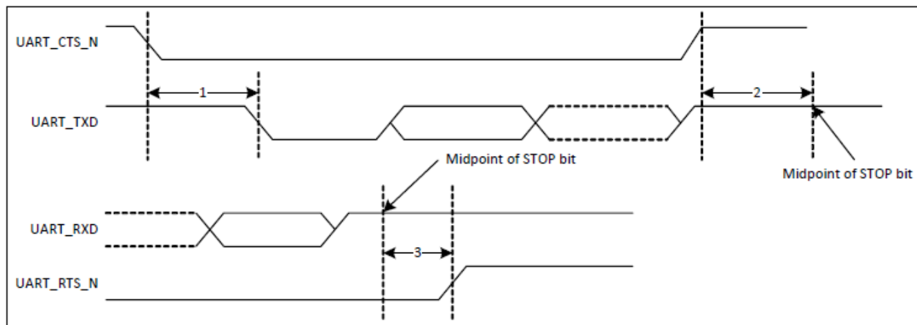
Figure 20 UART Timing
