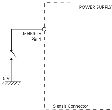
Remote On/Off (Inhibit) Figure 6
