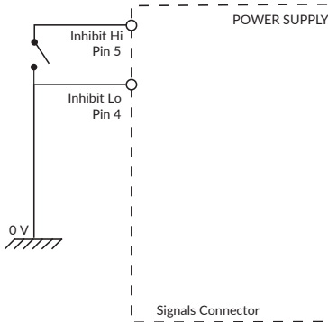
Remote On/Off (Enable) Figure 7
